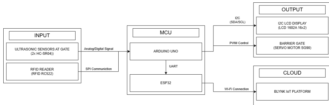
Figure 1: Proposed Smart Parking System Block Diagram
